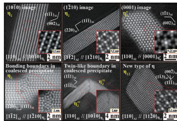
▲ 航太級鋁合金之原子級析出物相變態顯微結構演化機制 Microstructure evolution of atomic-level precipitates in aerospace-grade aluminum alloys
