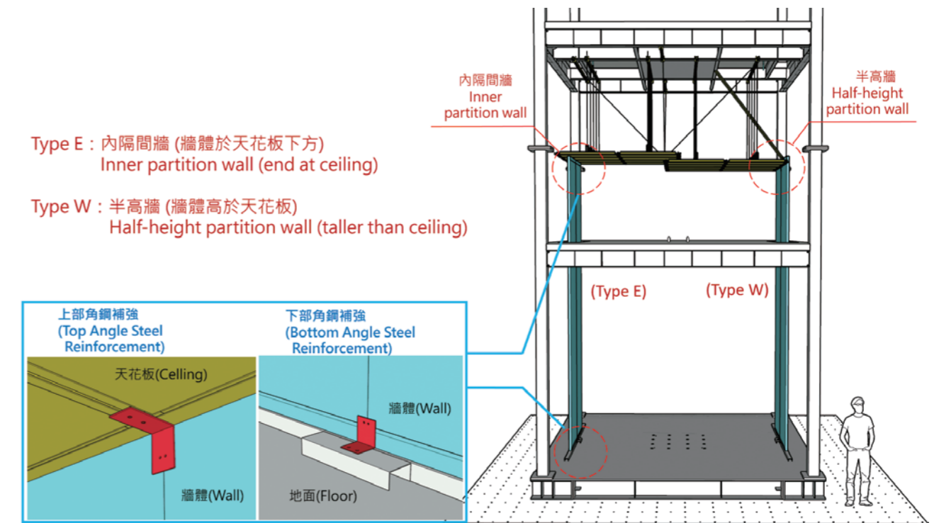
▲ 兩個獨立的系統同時試驗的耐震研究 Simultaneous testing of two systems for seismic studies
