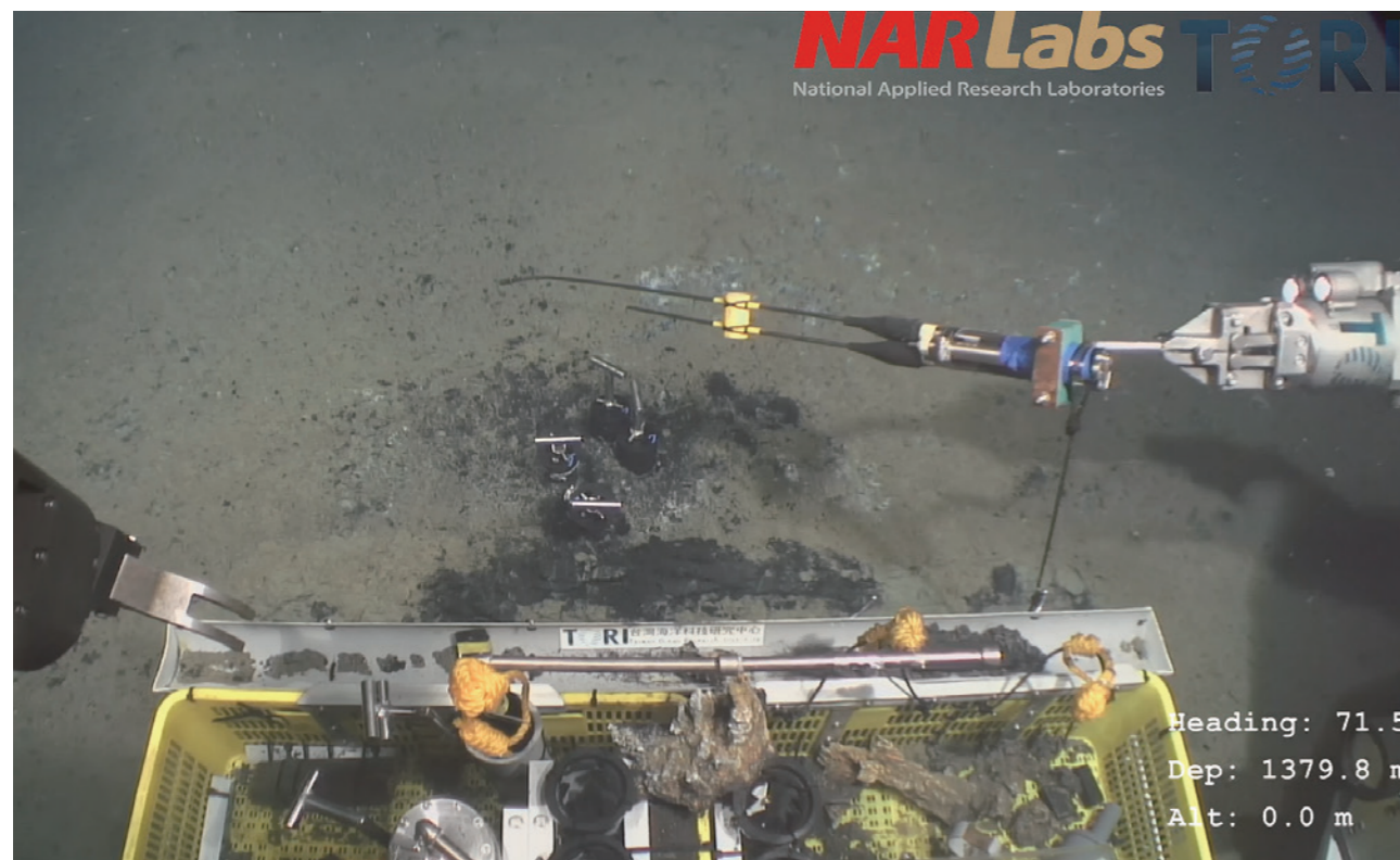
▲ ROV 執行地熱測量 ROV performs geothermal measurements
